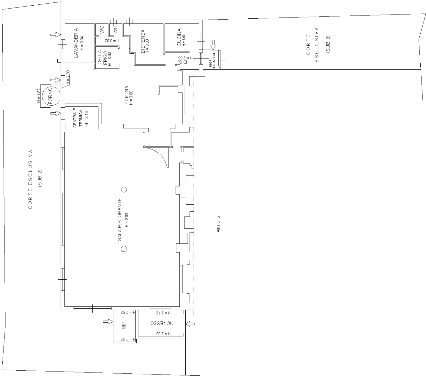
PIANO TERRA
