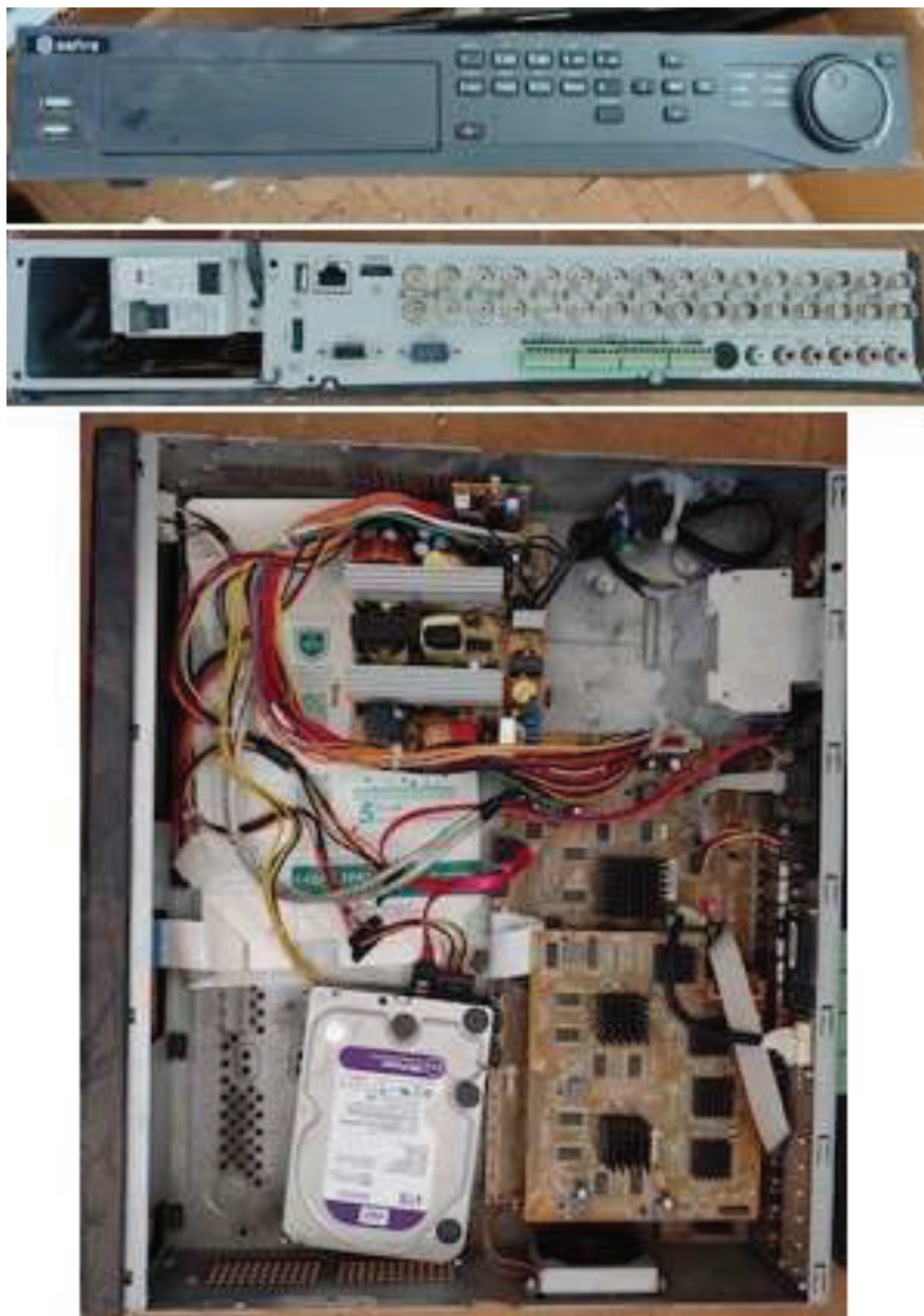
Foto 8 – DVR SAFIRE
